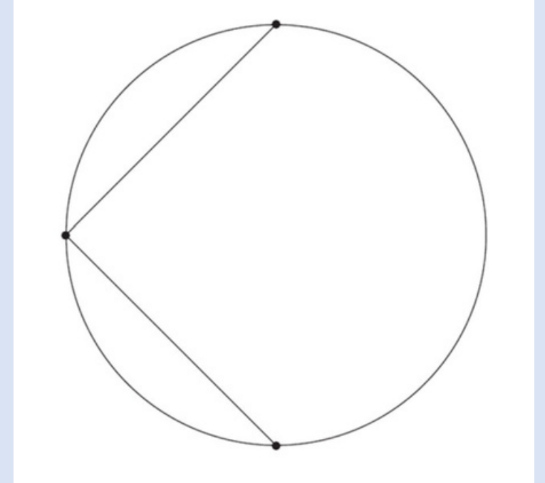
90° First quarter Square
