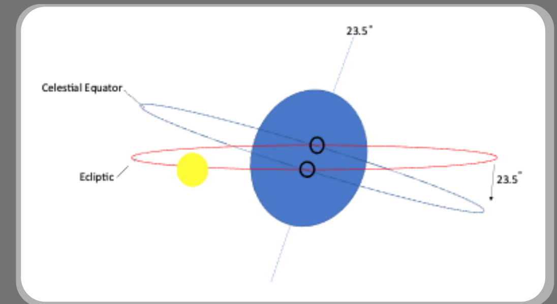
There are two natural intersection points between the C.E and the ecliptic
