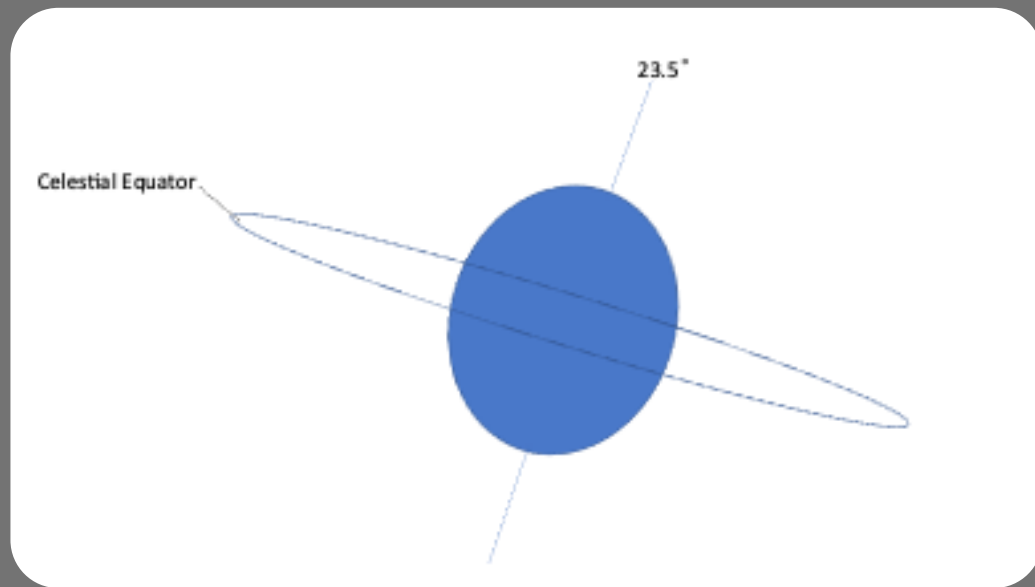
Plane of the equator of the earth extended outwards.
