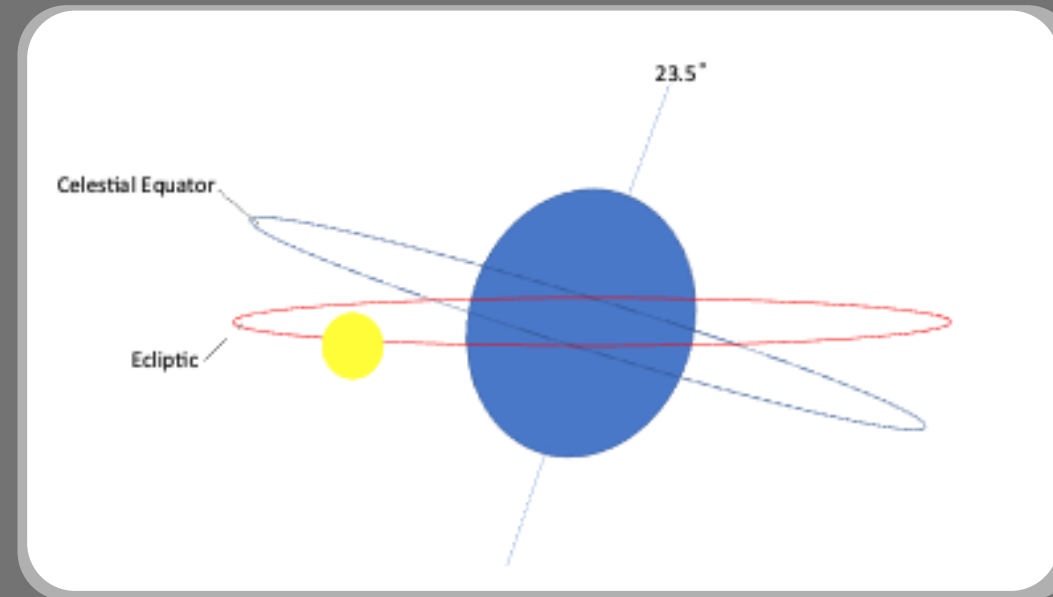
Ecliptic is the "apparent" path of the Sun. The celestial equator is tilted 23.5 degrees relative to the ecliptic
