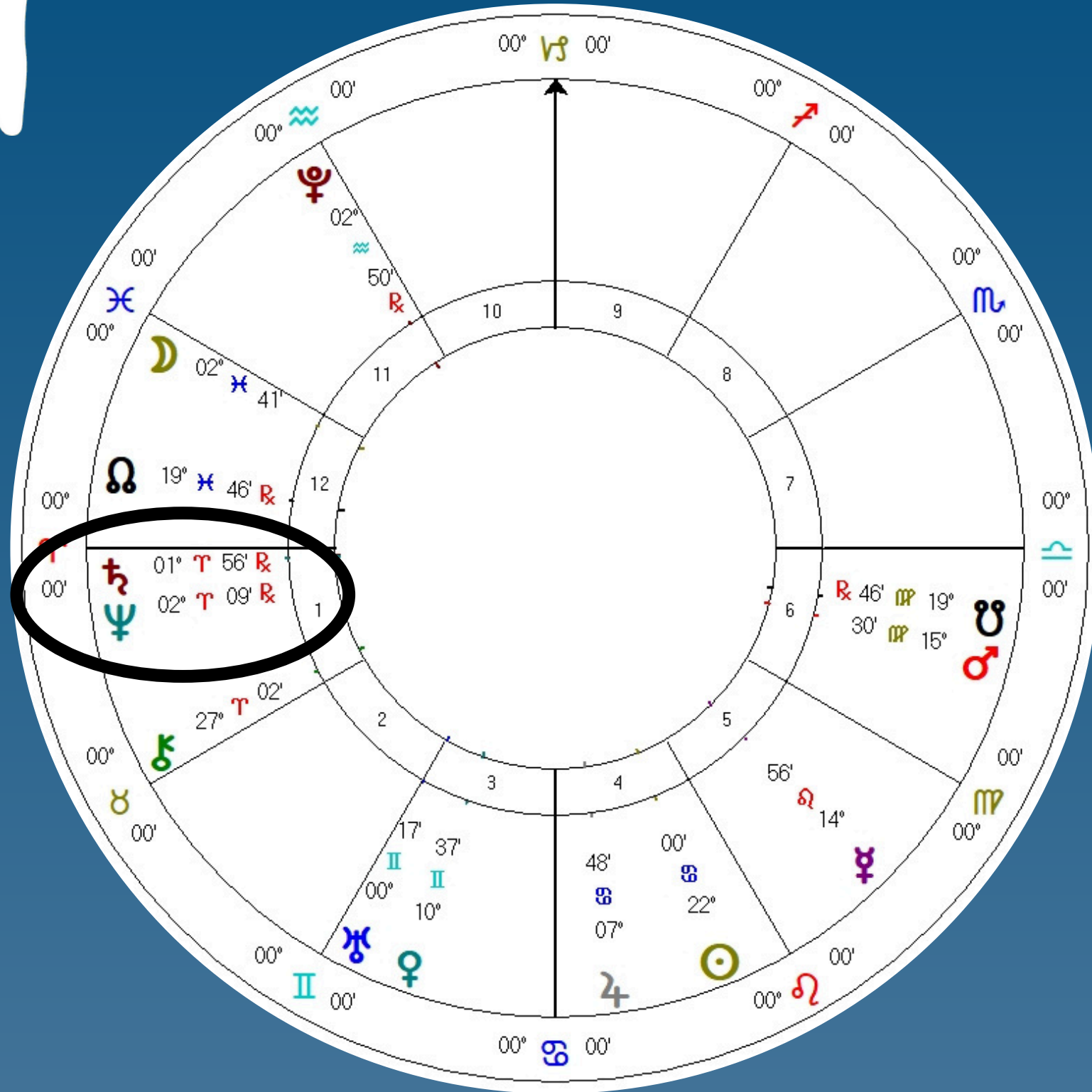
Saturn Neptune station Rx first half of July
